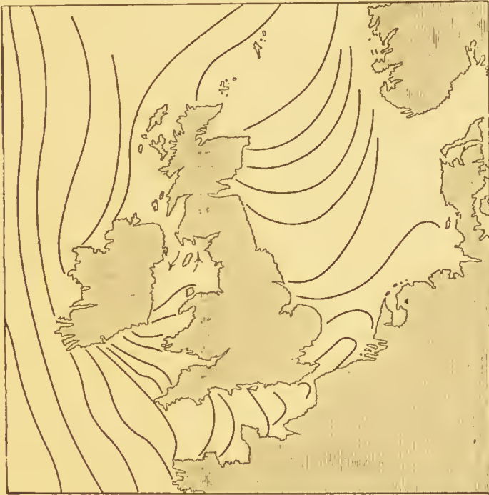
FIG. 109.—Co-tidal lines, showing the way tidal waves reach the Brit'sh Isles.
